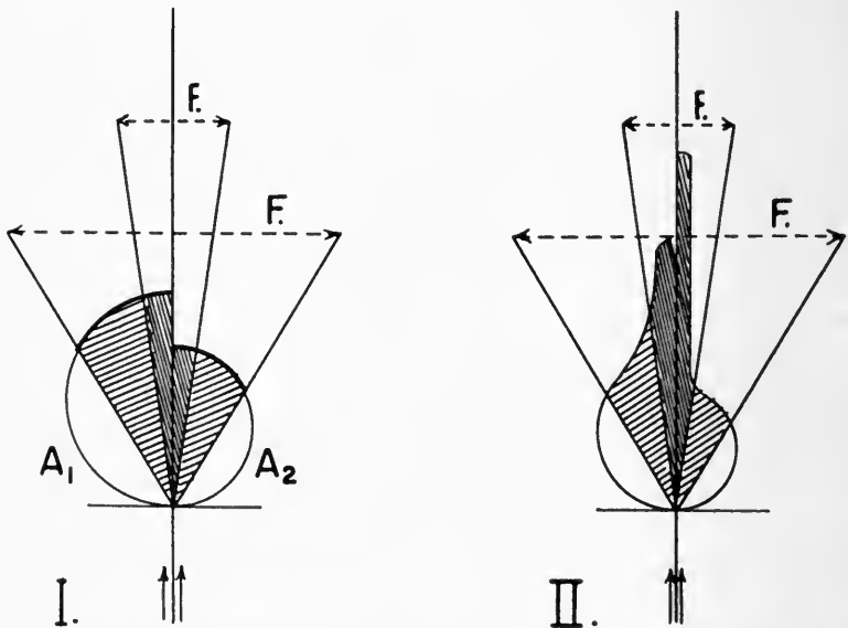
FIG. 10. A schematic demonstration of the influence of scattering upon observations with two different apertures: (I) the situation arising for a perfectly scattering emulsion; (II) for an imperfectly scattering emulsion.
